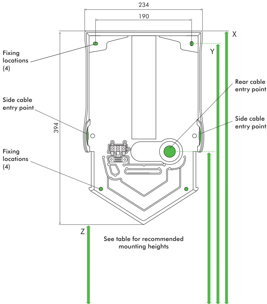
REAR ELEVATION
